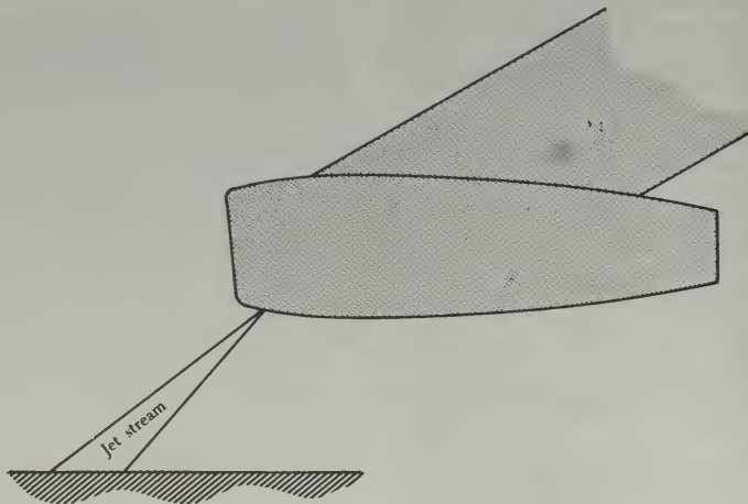
FIGURE 2-43. Inlet vortex destroyer jet stream.
